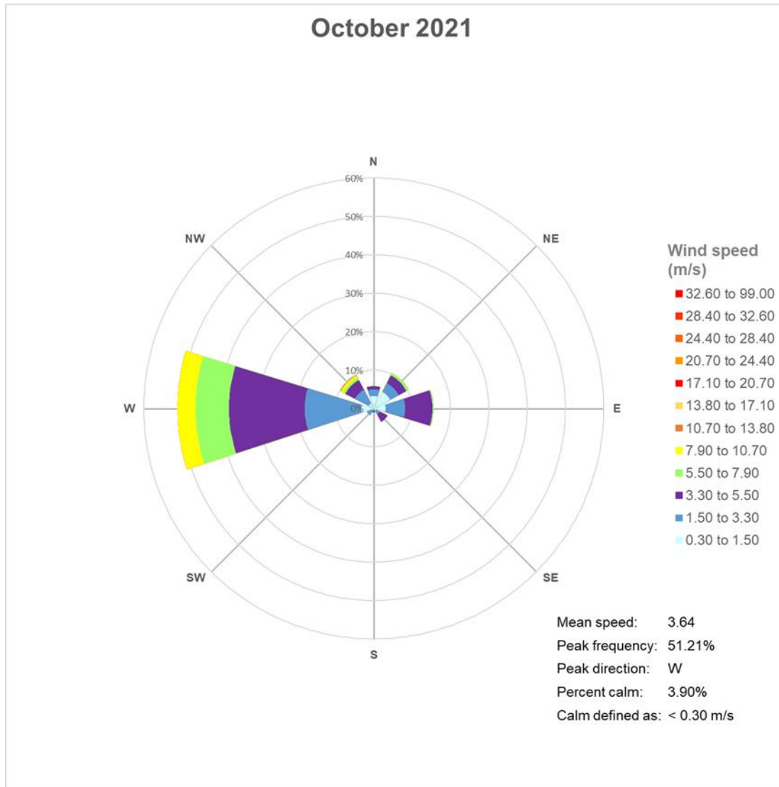
Figure 1. Wind rose data – October 2021
