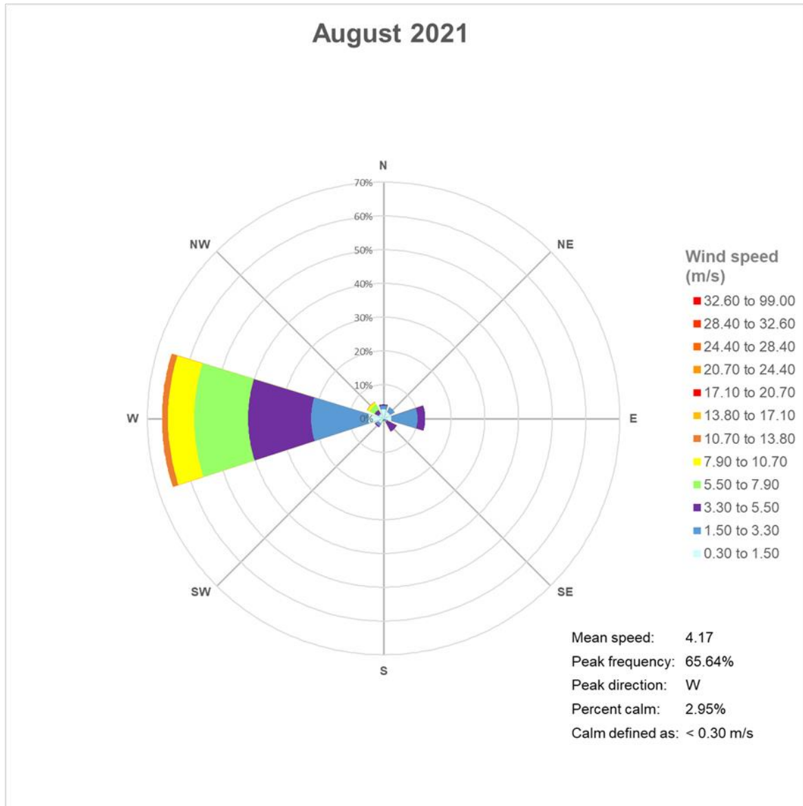
Figure 1. Wind rose data – August 2021
