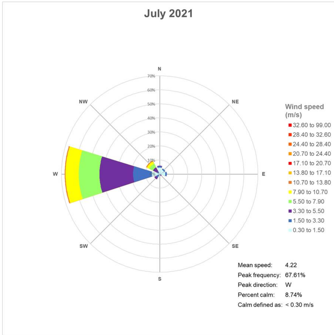
Figure 1. Wind rose data – July 2021
