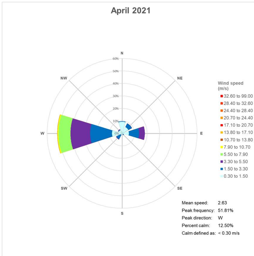
Figure 1. Wind rose data – April 2021
