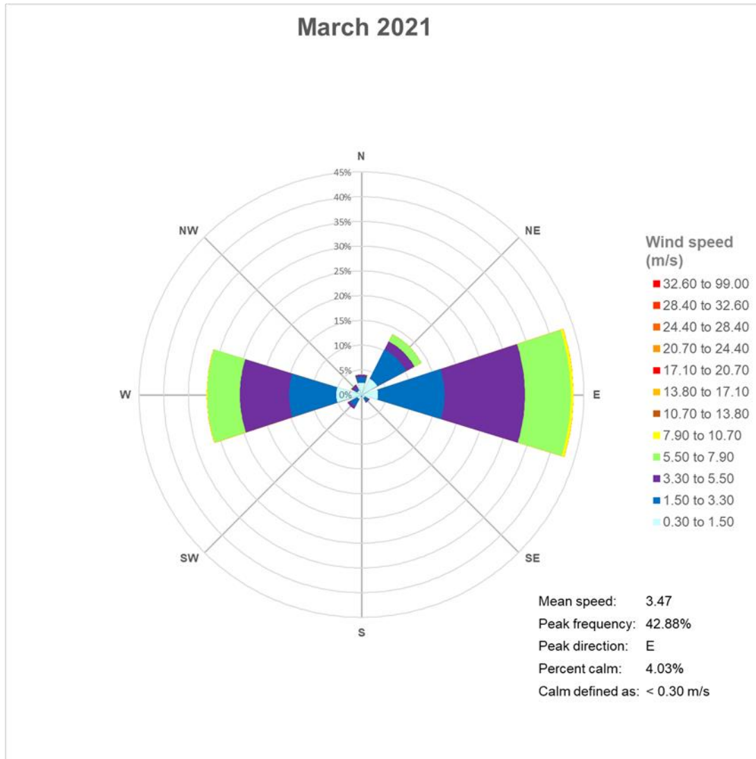
Figure 1. Wind rose data – March 2021
