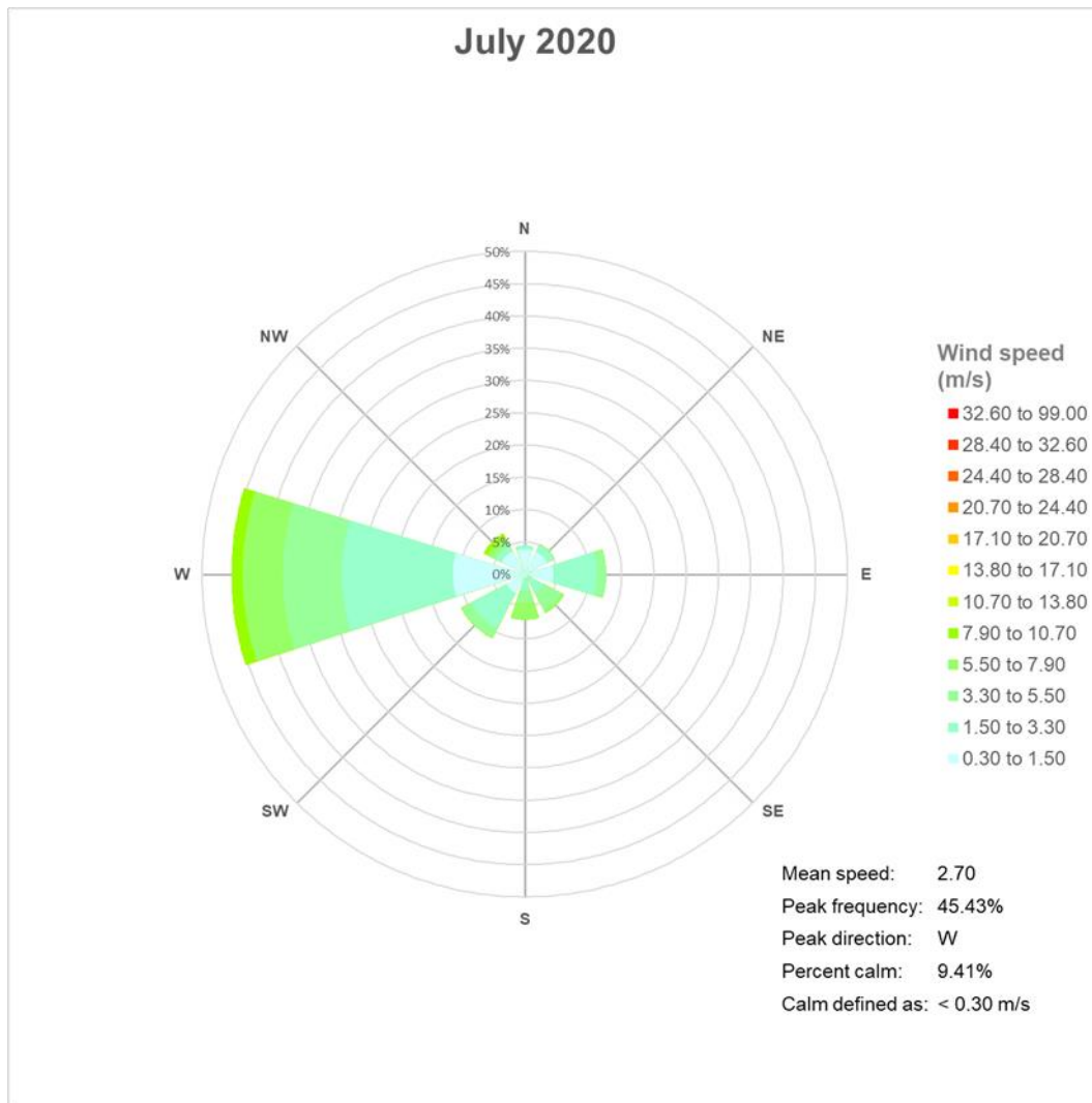
Figure 1. Wind rose data – July 2020
