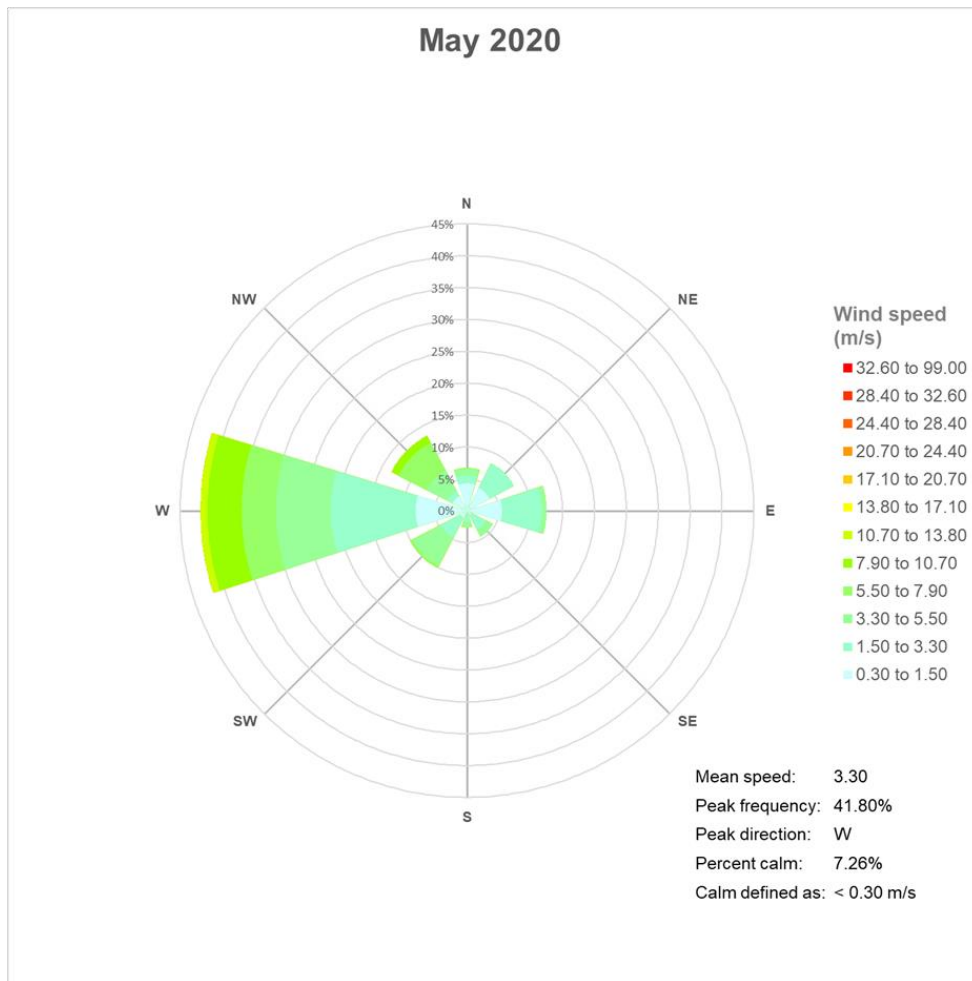
Figure 1. Wind rose data - May 2020
