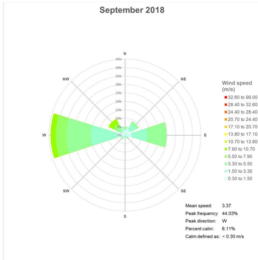
Figure 1. Prevailing wind direction (percentage for month) June - September 2018
