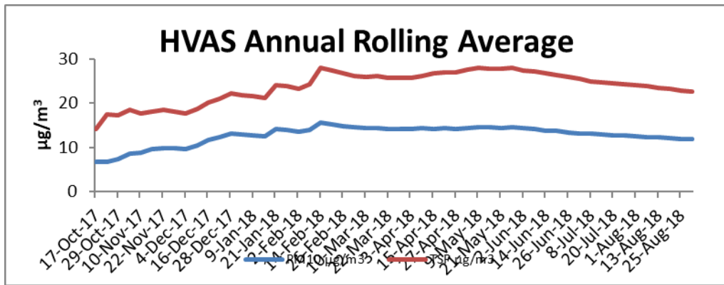
Figure 5. PM 10 and TSP annual rolling average results
