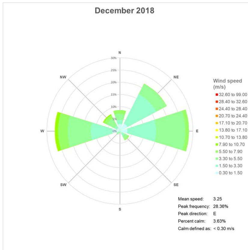
Figure 1. Prevailing wind direction (percentage for month) October - December 2018
