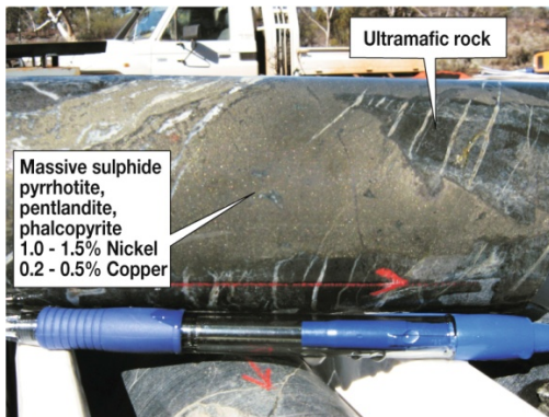
Example of Nickel Sulphide Bands in Avoca Downs Core
