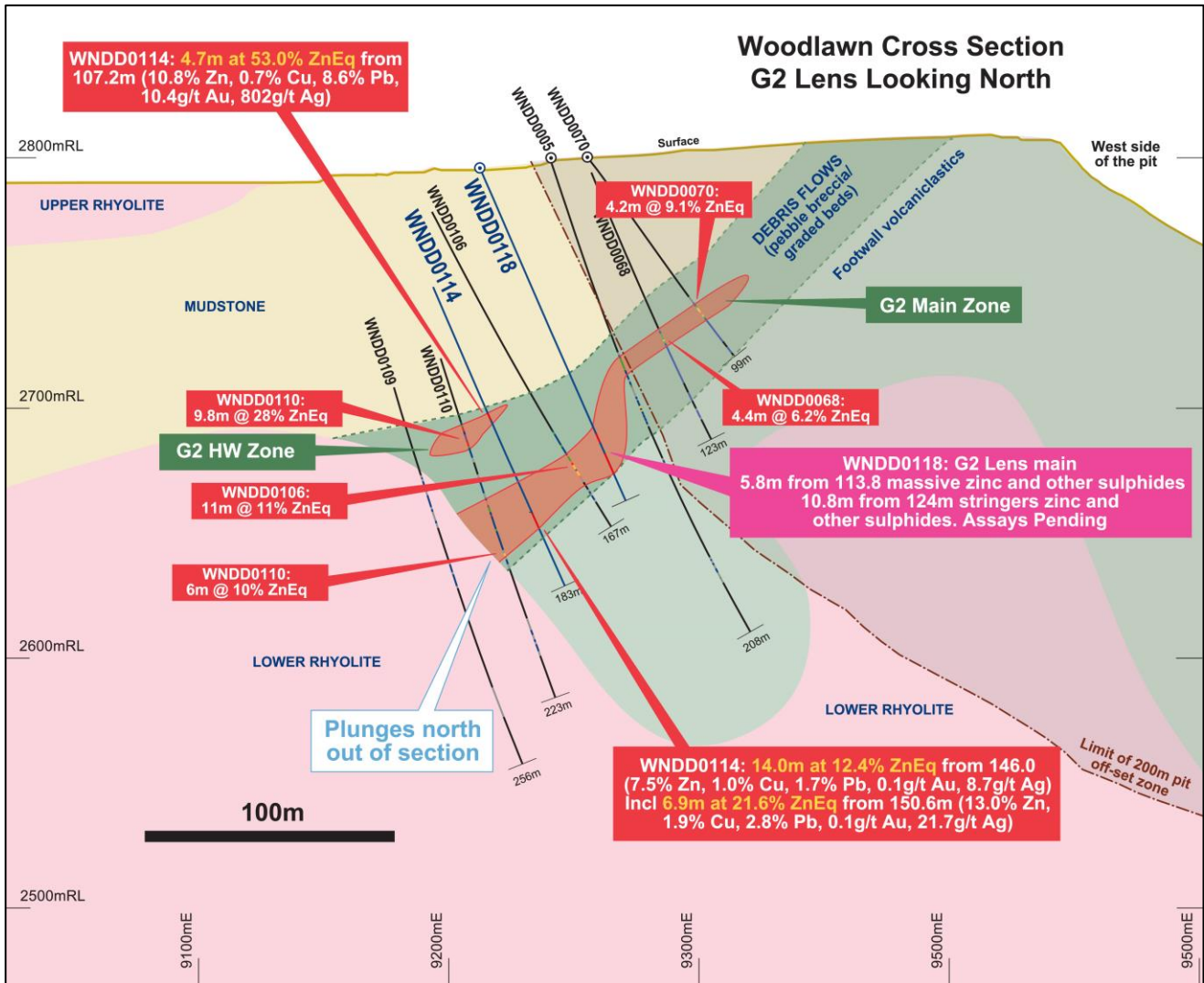
Figure 2: G2 Lens cross-section showing location of WNDD0114 in relation to previous drilling.
