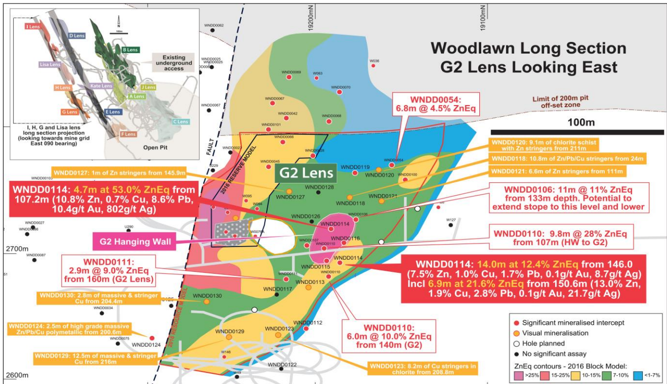
Figure 3: Woodlawn G2 Lens long-section showing interpreted lens shape, recent drilling and proposed infill holes.
